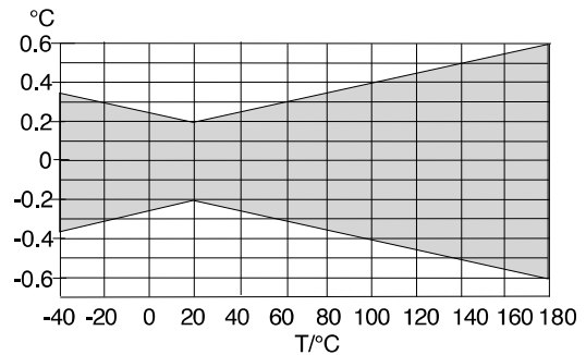
Temperature accuracy over the measurement range
