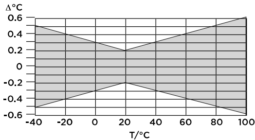
Temperature accuracy over measurement range
