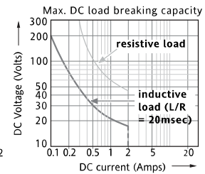
Graph 2 DC ratings
