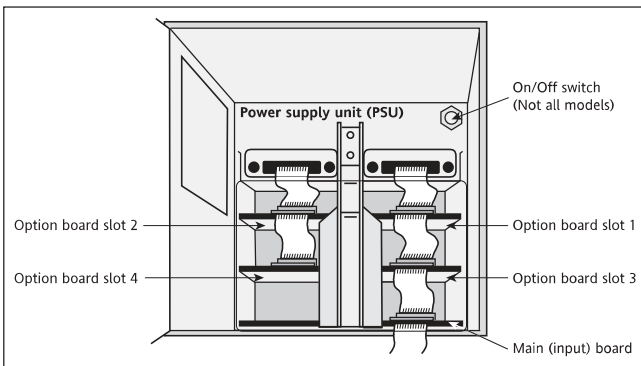
Exploded view
