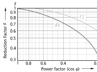
Graph 1 Derating curves
